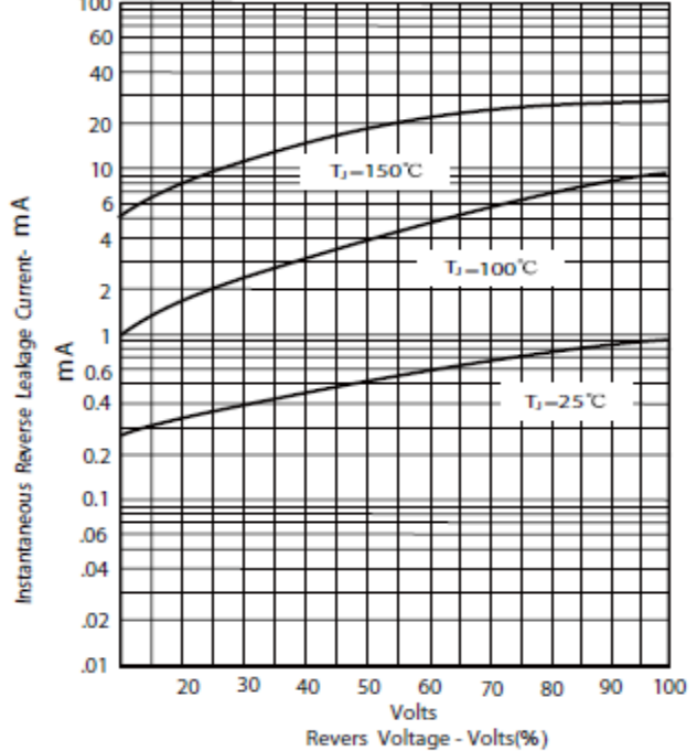
Figure.4-Typical Reverse Characteristics
